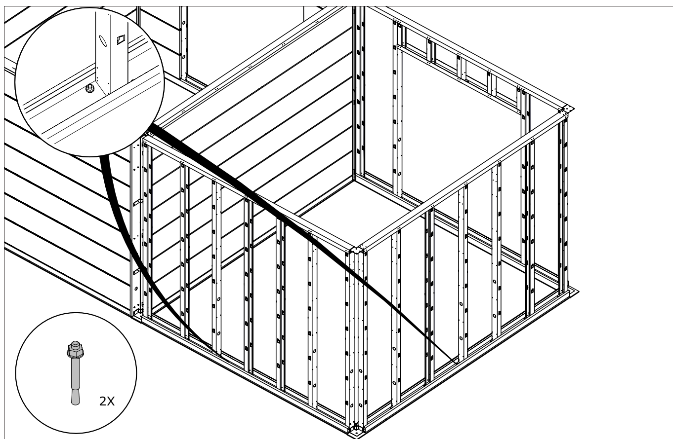
B1/B2/CD1/D2 Ancrage / Verankering / Anchoring / Verankerung
