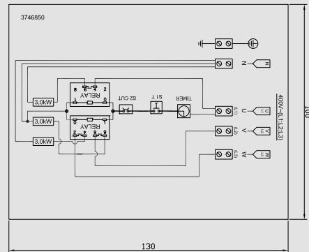
9 kW sauna stove with internal controller
